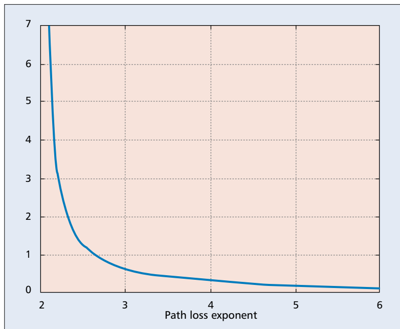
Figure 2. Normalized interference vs. path loss exponent.
