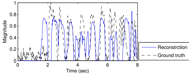
Fig. 3. Reconstructed audio sequence (solid) against the reference from the clean audio sequence (dashed).
