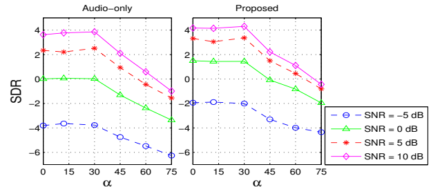
Fig. 5. The SDRs at different SNR levels.
