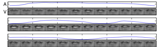
Fig. 2. The AV atoms obtained by the dictionary learning.
