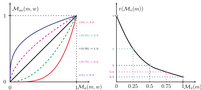
Fig. 1. Visually constrained TF mask generation.
