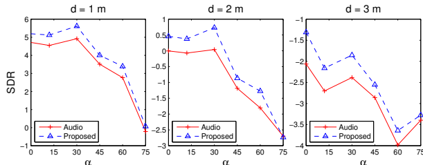
Fig. 4. The SDRs at different source-microphone distance.
