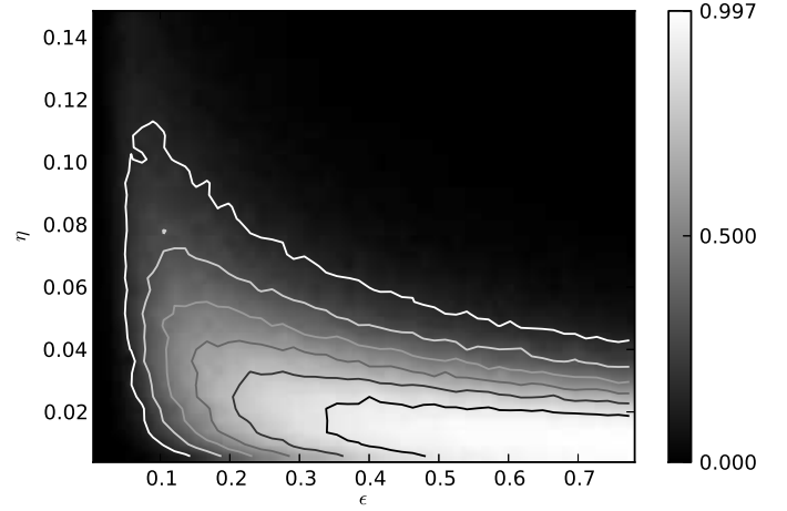
Fig. 5: Behaviour of \mathbf{IC} for a compressed sensing scenario matrix with a Gaussian measurement matrix and the Fused Lasso regularization. Empirical probability of the event \mathbf{IC} < 1 as a function of the parameter \varepsilon \in [1/N, 200/N] and the support size \eta \in [0.025, 0.15] .
