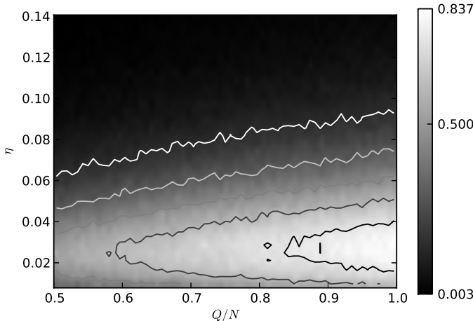
Fig. 4: Behaviour of \mathbf{IC} for a compressed sensing scenario matrix with a Gaussian measurement matrix and the Fused Lasso regularization. Empirical probability of the event \mathbf{IC} < 1 as a function of the sampling ratio Q/N \in [0.5, 1] and the support size \eta \in [0.025, 0.15] .
