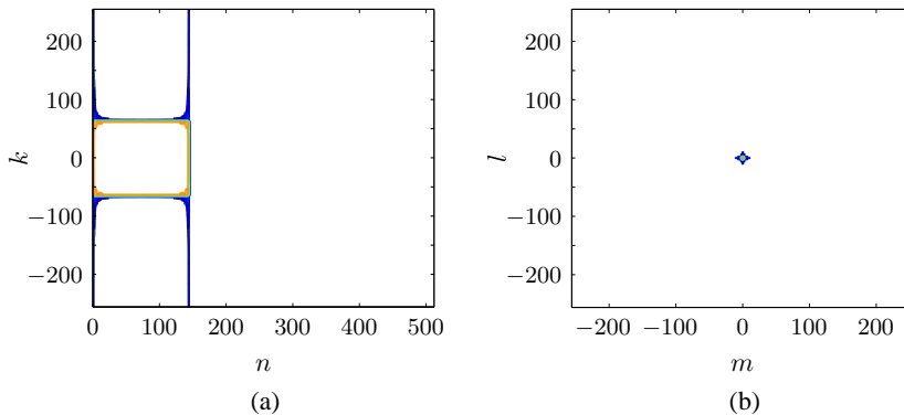
Fig. 1. TF representation of the OFDM process X[n] : (a) Real part of RS \bar{R}_X[n, k] , displayed for (n, k) \in [N] \times \{-N/2, \dots, N/2 - 1\} , with N = 512 ; (b) magnitude of EAF \tilde{A}_X[m, l] , displayed for (m, l) \in \{-N/2, \dots, N/2 - 1\}^2 .
