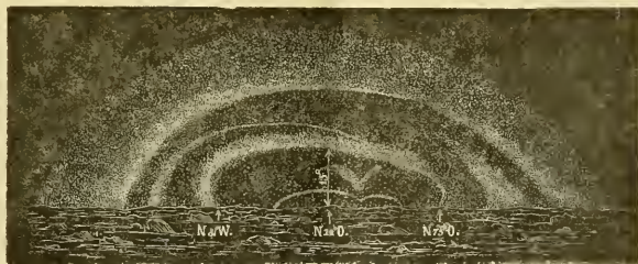
FIG. 2.—Auroral Arcs, Nordenskjöld.
