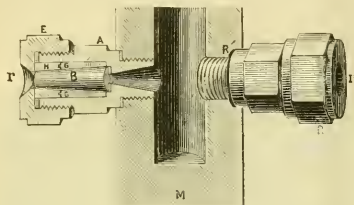
FIG. 2.—Details of apparatus in Fig. 1.
