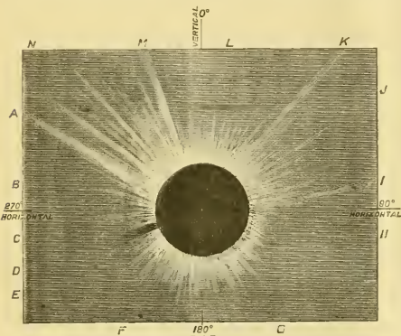
Corona as observed during solar eclipse of September 9, 1885, as seen from Taharaiti, North Island, New Zealand, about 40 miles north of centre line of totality:—A, 350' ; longest ray, 2-3 diams. B, first contact about 285' (vague). C, Sun apparently reappears about 260' (vague). D, 250' ; dark rift in corona. E, approximate position of large red protuberance which shot out just before close of totality. F, corona, \frac{1}{2} diam., rather ragged. G, corona, \frac{1}{2} diam., regular. H, large sun-spot with faculae close to the limb at time of first contact. I, 80' ; 3rd longest ray, \frac{1}{2} diam. J, between these two long rays corona extends nearly \frac{1}{2} diam., with some longer rays. K, longest ray, \frac{1}{2} diam. L, corona, hardly \frac{1}{2} diam. M, 2nd longest ray, \frac{1}{2} diam. N, between longest rays corona extends \frac{1}{2} to 1 diam.; 2 long rays \frac{1}{2} diam. (N.B.—Corona alone was observed; relative position and lengths of rays reliable; absolute lengths to be taken with caution.)
