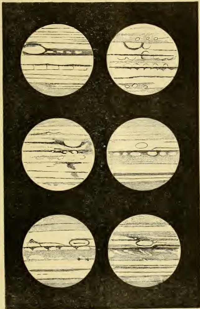
FIG. 1.—Probably recurrent markings on Jupiter. I. 1857, November 27 (Dawes). II. 1859, December 20, 10h. 50m. (Huggins). III. 1858, March 2, 9h. (Huggins). IV. 1870, January 23, 8h. 20m. (Gledhill). V. 1872, February 2, 10h. 50m. (Gledhill). VI. 1885, February 25, 12h. 50m. (Denning).
