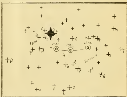
Diagram exhibiting the displacement in the radiant point amongst the stars of Hercules and Lyra on the nights of April 18, 19, and 20, 1885.
