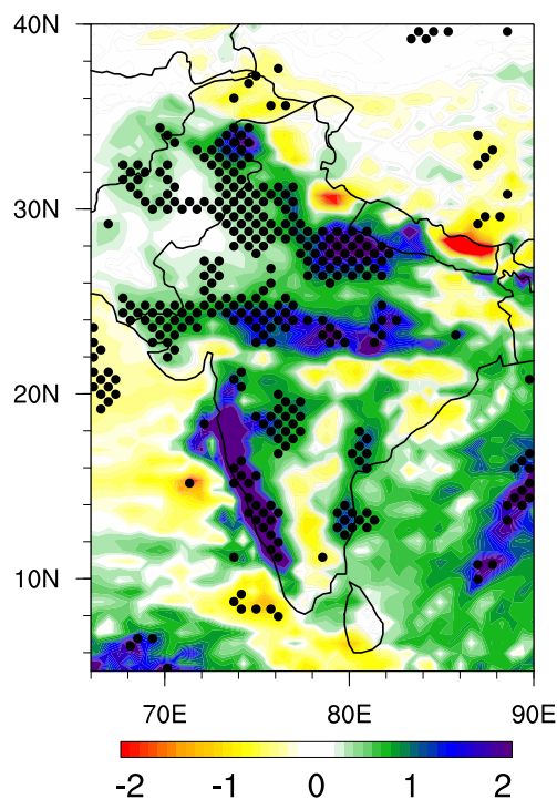
Figure 6. Spatial pattern of WRF-Chem ensemble mean differences in rainfall ( \text{mm day}^{-1} ) between ALLF and NDST experiments during JJA 2008. Areas that have a 90% confidence level based on a one-sided Student's t test are indicated by dots.
