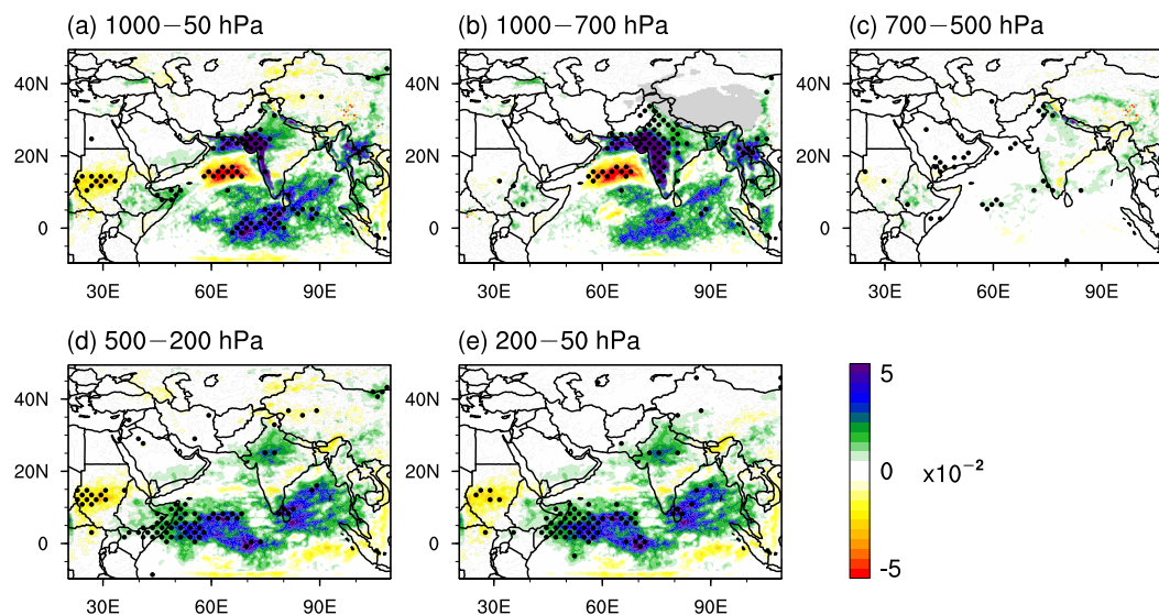
Figure 12. Spatial patterns of the ensemble means of cloud fraction responses (ALLF minus NDST; scale factor: 10^{-2} ) for JJA 2008 between various atmospheric layers. The dots indicate where cloud fraction responses have a 95 % confidence level based on a one-sided Student's t test.
