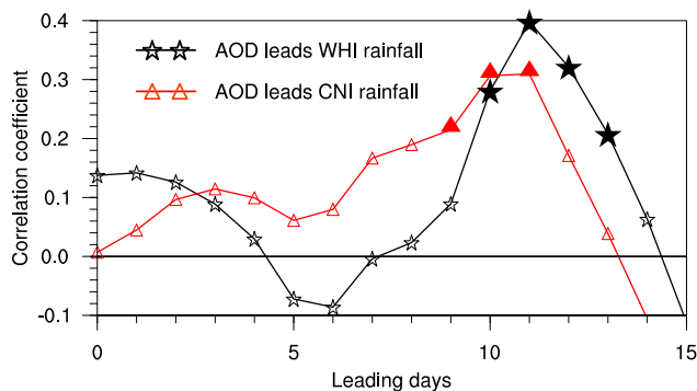
Figure 10. Cross-correlation coefficients between WRF-Chem simulated rainfall responses in WHI and CNI and dust AOD (ALLF minus NDST) in remote DST regions. All correlations are calculated based upon daily anomalies obtained by subtracting the 21-day running mean from the daily data. The filled markers represent that the correlation coefficients with a 95 % confidence level based on the t test. The unfilled markers are not significant.
