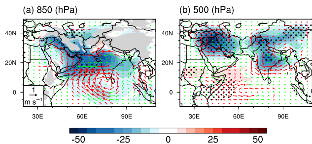
Figure 16. Spatial patterns of WRF-Chem ensemble mean differences in GPH (shading; unit: m) and winds (arrows; units: \text{m s}^{-1} ) at (a) 850 hPa and (b) 500 hPa between ALLF and NDST experiments. The dotted areas show a 95 % confidence level based on a one-sided Student's t test. The red arrows show wind differences that have a 95 % confidence level based on a one-sided Student's t test, and green arrows are other wind differences (no confidence).
