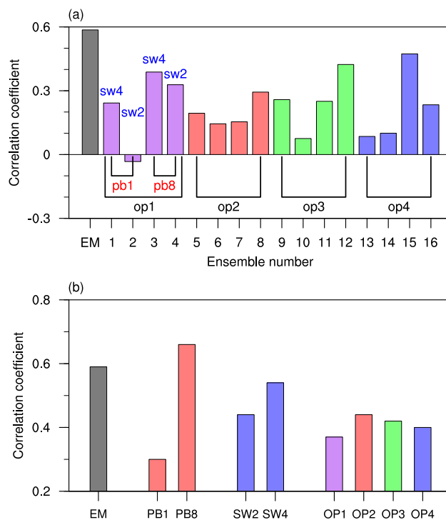
Figure 7. The spatial correlation coefficients between the regressed rainfall change pattern (Figure 5c) and the modeled rainfall response (Fig. 6) in (a) each ensemble member (marked by numbers from 1 to 16), their ensemble mean (marked by “EM”), and (b) the ensemble means of several subgroups of the ensemble members. “EM” stands for the ensemble mean of all ensemble members. In (b), “PB1” and “PB8” indicate the ensemble means of the ensemble members in which PBL option 1 and 8 are used, respectively. “SW2” and “SW4” indicate the ensemble means of the ensemble members in which SW option 2 and 4 are used, respectively. “OP1”, “OP2”, “OP3”, and “OP4” indicate the ensemble means of the ensemble members in which aerosol chemical mixing rules 1, 2, 3, and 4 are used, respectively. The region for calculating the spatial correlation is WHI. Using other figures in Fig. 5 for the evaluations gets similar results. See Table 2 for the denotations.
