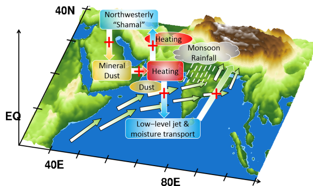
Figure 18. Schematic diagram shows the physical mechanism for the Middle East dust–ISM rainfall connection. Red plus signs represent positive responses. The positive feedback between dust emissions, atmospheric heating, and shamal winds is seen as a cycle over the Middle East and the Arabian Sea.
