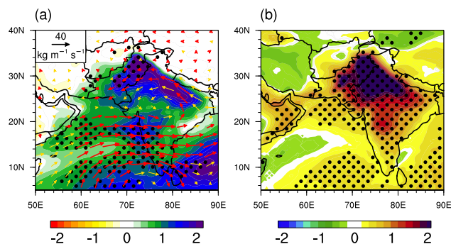
Figure 17. Spatial patterns of WRF-Chem ensemble mean differences in (a) precipitable water (shading; unit: mm) and water vapor flux (arrows; units: \text{kg m}^{-1} \text{s}^{-1} ) both integrated within the entire atmospheric column and (b) moist static energy (units: \text{kJ kg}^{-1} ) in the three lowest model layers. Black dots represent the differences in precipitable water and moist static energy that have a 95 % confidence level based on a one-sided Student's t test. The red arrows represent wind differences that have a 95 % confidence level, and the gold arrows represent other wind differences (no confidence).
