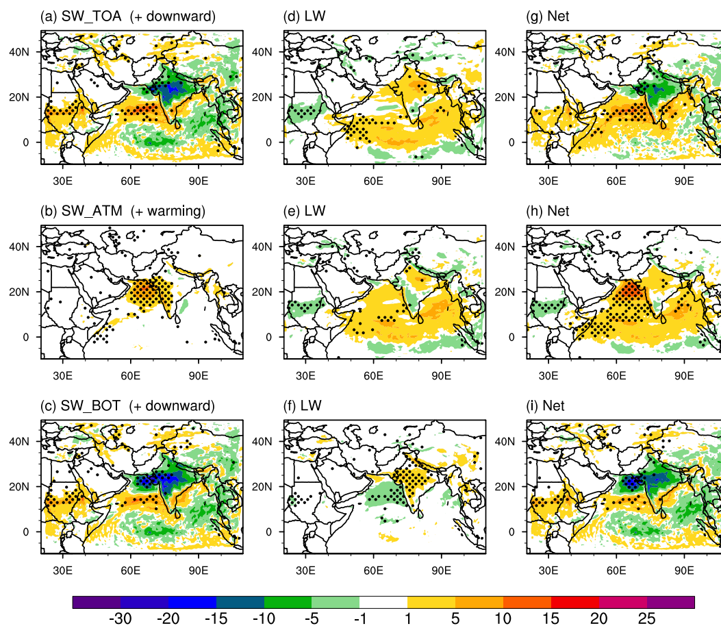
Figure 13. Same as Fig. 11, but for radiative effects ( \text{W m}^{-2} ) at cloudy conditions, calculated as radiative effects at all-sky conditions minus those at clear-sky conditions.
