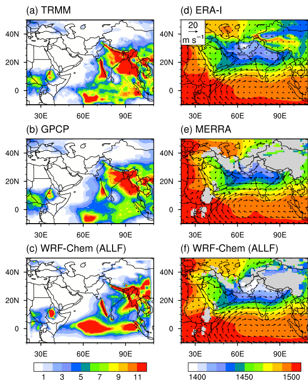
Figure 2. Left: precipitation ( \text{mm day}^{-1} ) from (a) TRMM, (b) GPCP, and (c) WRF-Chem (ALLF). Right: 850 hPa GPH (shading; unit: m) and wind (arrows; units: \text{m s}^{-1} ) from (d) ERA-I, (e) MERRA, and (f) WRF-Chem (ALLF). All variables are average for JJA 2008. In (e) and (f), topography is marked out in gray.
