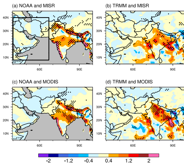
Figure 5. Same as Fig. 4, but for the spatial patterns of precipitation ( \text{mm day}^{-1} ) regressed on area-averaged AOD in the AS, the south AP, and the IP (box in a ).
