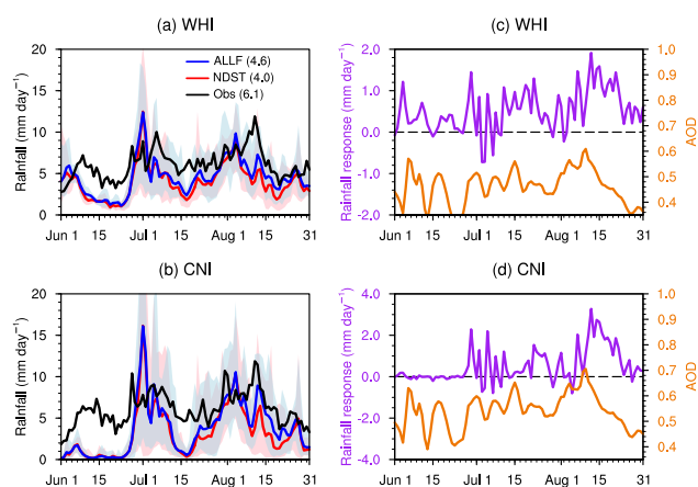
Figure 9. Left: time series of rainfall ( \text{mm day}^{-1} ) in ensemble means of ALLF and NDST experiments and rainfall spread of all 32 ensemble members. Right: ensemble mean rainfall responses ( \text{mm day}^{-1} ) in WHI, and CNI and AOD in DST (from ALLF). Light blue and red colors represent the spread of rainfall in ALLF and NDST members, respectively. The numbers in parentheses are time-averaged rainfall.
