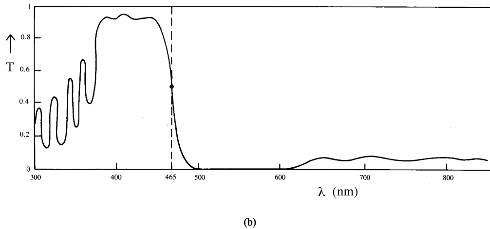
Figure 2.19. Schematic transmission curves of the V_T (a), and B_T (b) star mapper channels.
