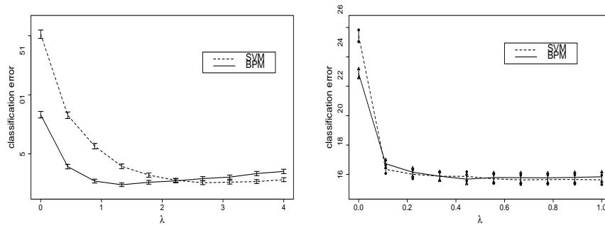
Figure 2: Generalisation error versus \lambda for a to y problem using linear kernels (left) and for the heart dataset using RBF kernels with \sigma = 10.0 (right). The error bars indicate one standard deviation of the estimated mean.
