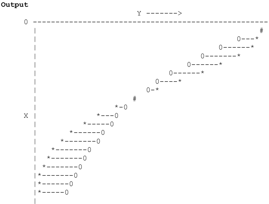
Fig.6.15 Plotting of two functions
