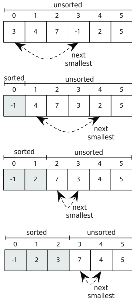
Figure 12—First few steps in selection sort
