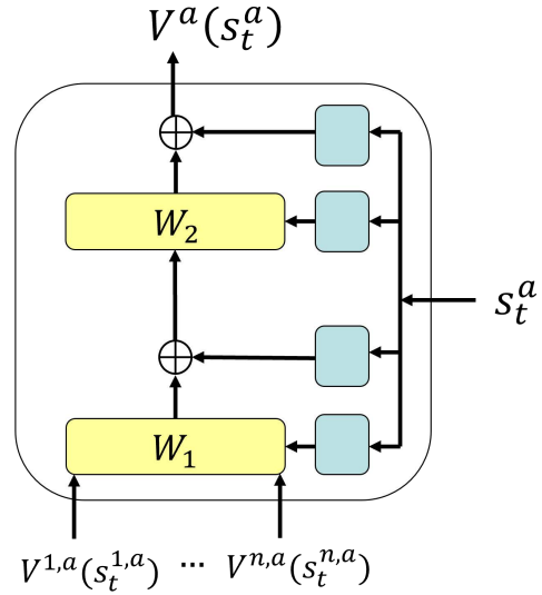
Figure 2: Hierarchical mixing network structure for solving RMP
