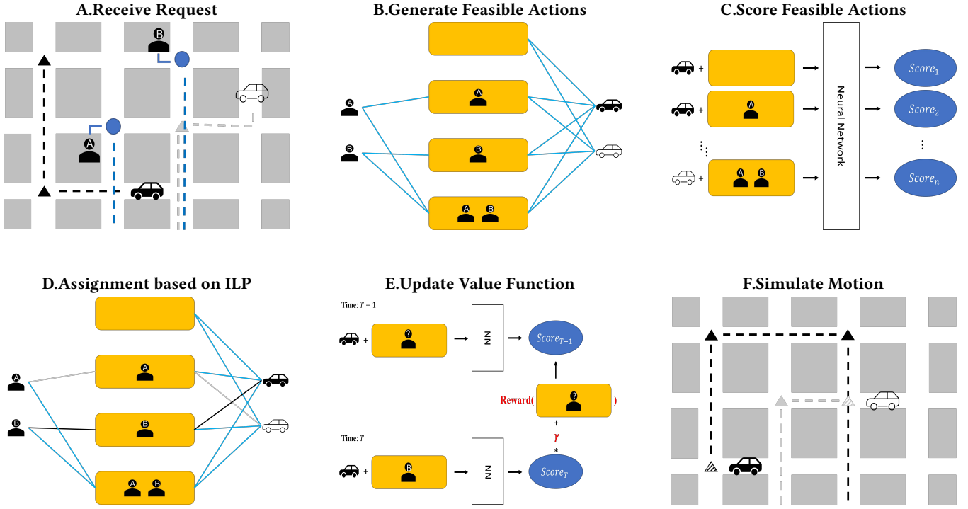
Figure 1: Outline of NeurADP approach for RMP
