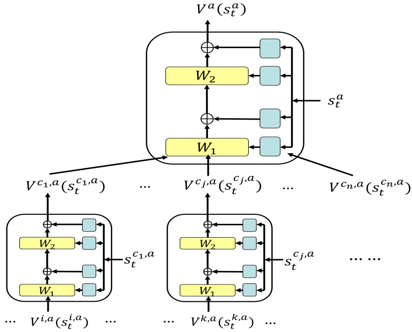
Figure 3: Hierarchical mixing network for solving RMP
