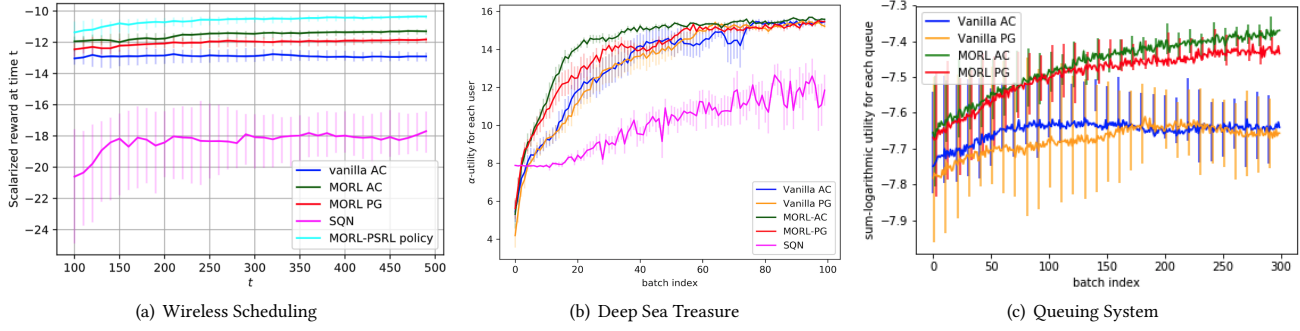
Figure 2: Learning curves for the three environments considered for the proposed algorithm against standard Actor Critic, Policy Gradient, and SQN algorithms. The proposed algorithm learns policies which maximizes the scalarized rewards in all three setups. (a) Wireless Scheduling: For this setup we plot the performance of the learned policies using multiple algorithms. (b) For the episodic Deep Sea Treasure problem, we compare the MORL-PG algorithm with Scalarized-DQN (SDQN) [35]. (c) For the queuing system we compare MORL-AC algorithm with MORL-AC, and their vanilla implementations.
