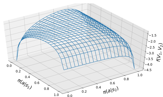
Figure 1: Proportional fairness for a 2 user, 2 state resource sharing process. The optimal strategy is not deterministic as the maximum does not lie on the boundary of the \pi(a|s_1) - \pi(a|s_2) grid.
