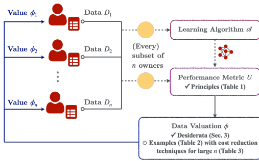
Figure 1: Overview of the data valuation problem with n data owners. The learning algorithm \mathcal{A} (e.g., logistic regression) takes in data and produces a model. The performance metric U (e.g., validation accuracy) used to evaluate the value of data/model is selected to follow certain principles. The data valuation strategy \phi (e.g., Shapley value [Sec. 3.2]) is selected to satisfy certain desiderata. We may consider the performance metric for multiple subsets of data owners and techniques to reduce the computational cost.
