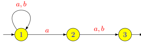
Figure 3.5. A nondeterministic automaton.
