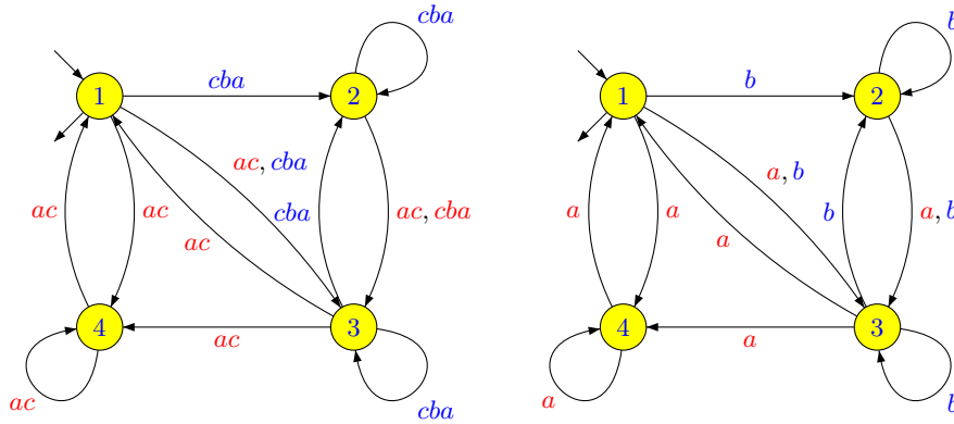
Figure 4.12. Computation of a nondeterministic automaton recognising \varphi^{-1}(L) .
