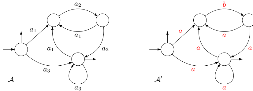
Figure 5.2. Construction of an automaton recognising [(ab)^*a]^* .
