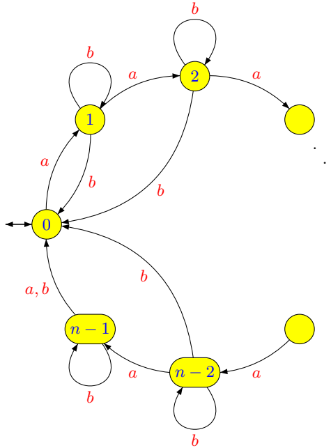
Figure 6.1. The automaton \mathcal{A}_n .
