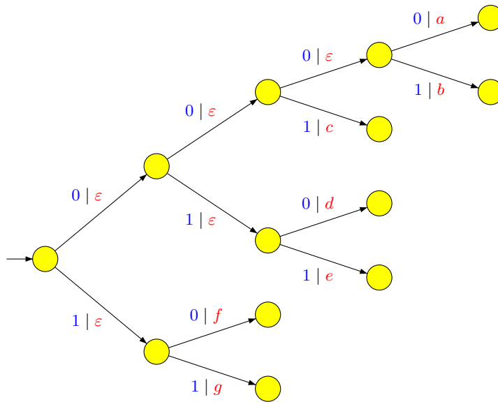
Figure 1.5. A pure sequential automaton realizing the decoding.
