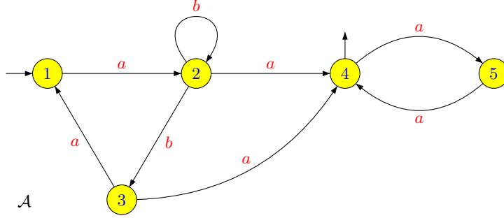
Figure 4.7. An automaton recognising L_1L_2 .
