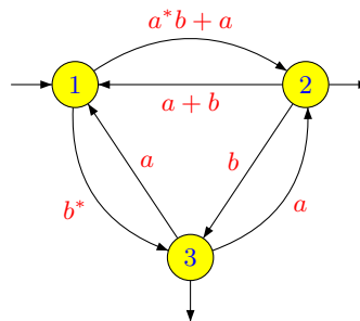
Figure 5.7. An extended automaton.
