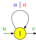
Figure 1.8. A sequential automaton realizing the function x \rightarrow uxv .
