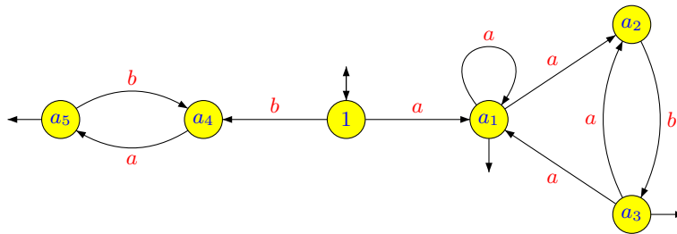
Figure 5.4. A nondeterministic automaton recognising L .
