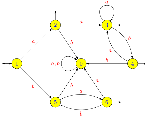
Figure 5.5. A deterministic automaton recognising L .
