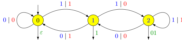
Figure 1.10. A sequential transducer realizing the multiplication by 3.
