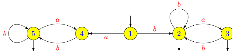
Figure 1.2. The minimal automaton of L .
