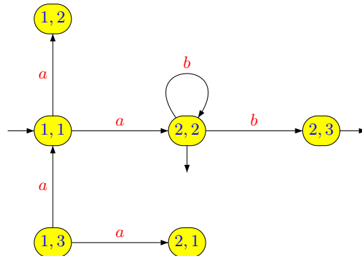
Figure 4.2. An automaton recognising L \cap L' .
