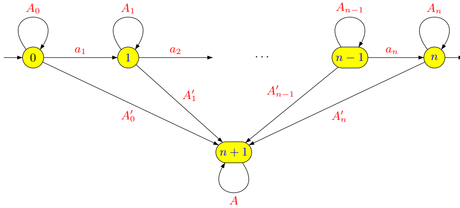
Figure 1.1. An automaton recognising L .
