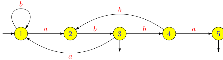
Figure 3.4. A deterministic automaton.
