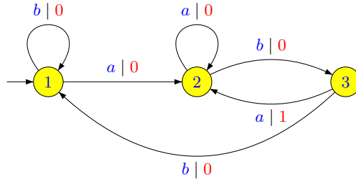
Figure 1.7. A function computing the number of occurrences of aba .
