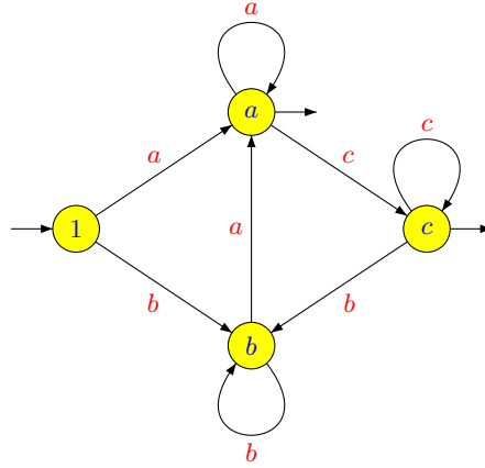
Figure 5.1. An automaton recognising a local language.
