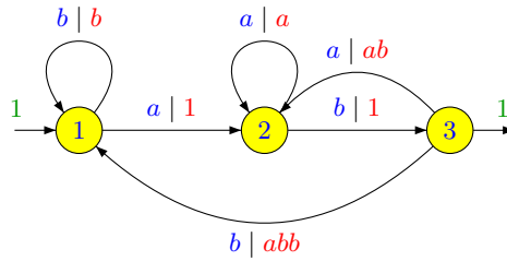
Figure 1.9. A sequential automaton realizing the function x \rightarrow x(ab)^{-1} .
