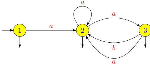
Figure 4.9. An automaton recognising L^* .
