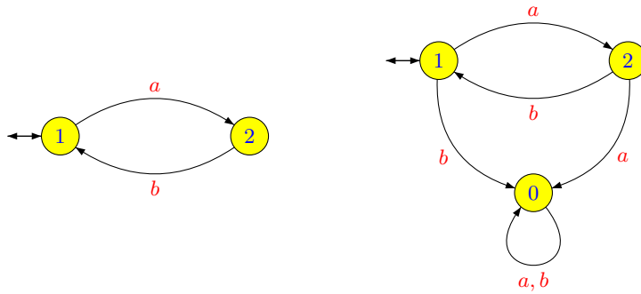
Figure 4.14. The minimal and minimal complete automata of (ab)^* .
