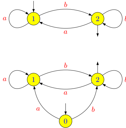
Figure 3.10. An automaton and its standardized version.
