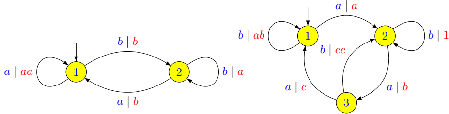
Figure 2.5. The automata \mathcal{A} (on the left) and \mathcal{B} (on the right).
