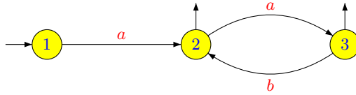
Figure 4.8. A standard automaton recognising L .
