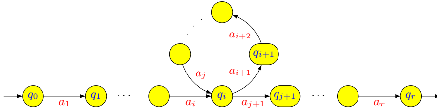
Figure 3.3. Illustration of the pumping lemma.
