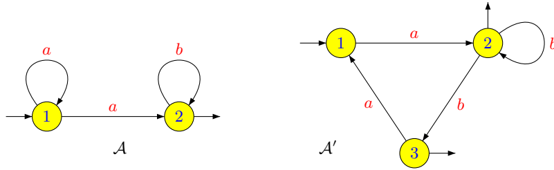
Figure 4.1. The automata \mathcal{A} and \mathcal{A}' .
