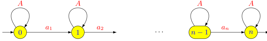
Figure 4.2. A nondeterministic automaton recognising L .
