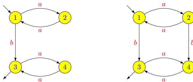
Figure 5.1. The minimal automata of K and L .
