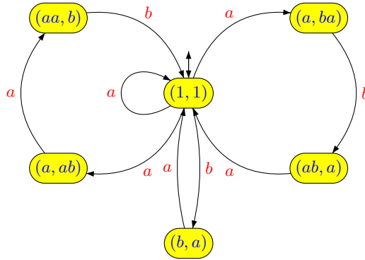
Figure 6.1. A flower automaton.
