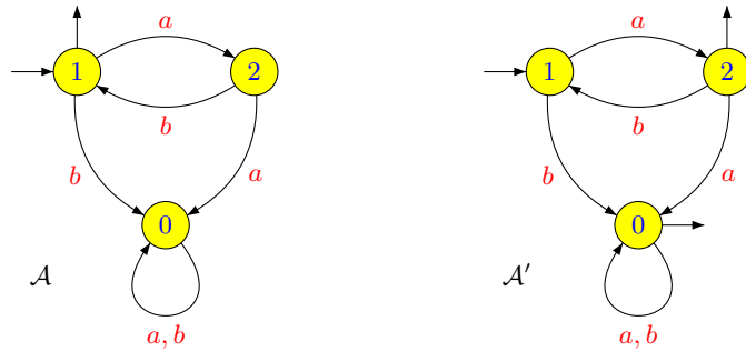
Figure 4.6. Complementation of a deterministic automaton.
