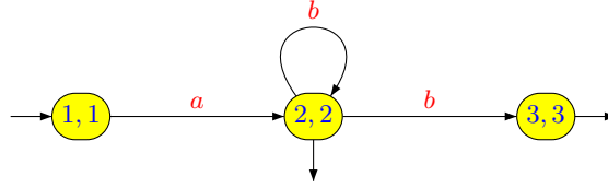
Figure 4.3. A trimmed automaton recognising L \cap L' .
