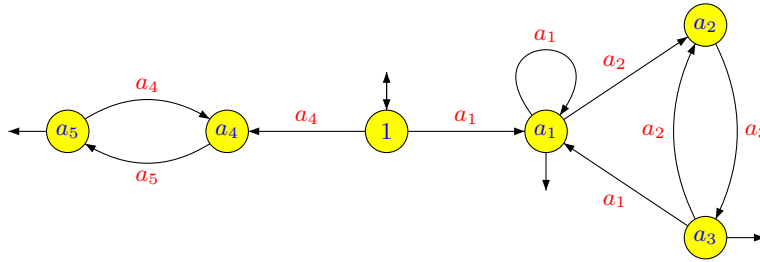
Figure 5.3. A local automaton recognising L' .
