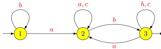
Figure 3.1. A deterministic automaton.
