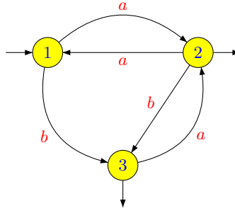
Figure 5.6. An automaton.
