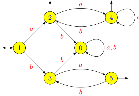
Figure 4.13. The minimal automaton of L .
