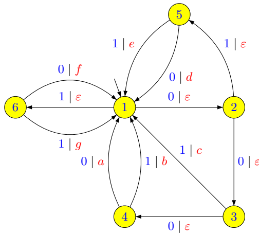
Figure 1.6. The same pure sequential automaton...
