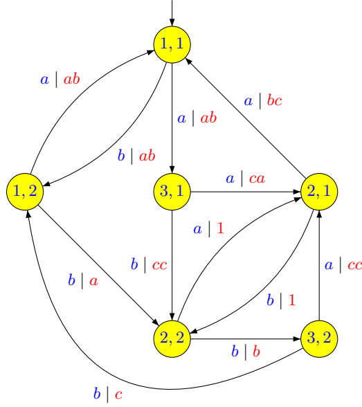
Figure 2.6. The wreath product \mathcal{B} \circ \mathcal{A} .
