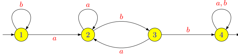
Figure 3.1. The minimal automaton of A^*abbA^* .
