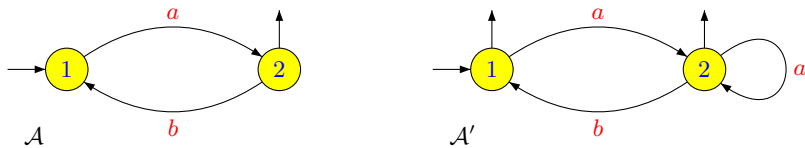
Figure 4.10. A nonstandard automaton \mathcal{A} and the automaton \mathcal{A}' .
