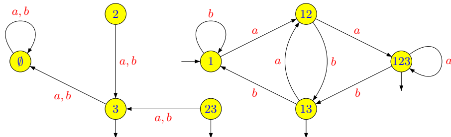
Figure 3.6. After determinisation...
