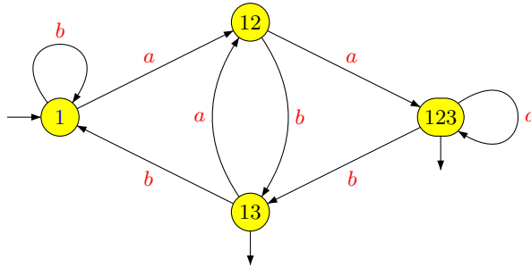
Figure 3.7. ... and trimming.
