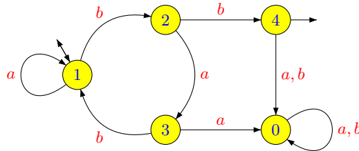
Figure 7.1. The minimal automaton of L .
