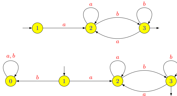
Figure 4.15. The minimal and minimal complete automata of aA^*b .
