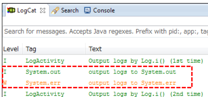
Figure 4.8-3 Difference of System.out/err in LogCat output, between development application and release application
