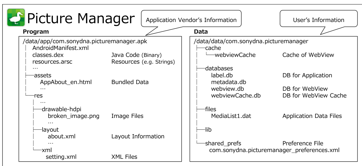
Figure 3.1-1 Information Contained in an Application
