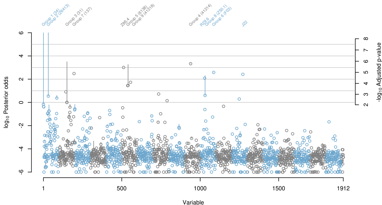
Figure 1 Individual variables (points) and pre-defined groups of variables (vertical lines) with the strongest evidence of direct effects on the risk of COVID-19 hospitalization in UK Biobank. Evidence was quantified simultaneously by \log_{10} posterior odds and -\log_{10} adjusted p -value using Doublethink. Groups were defined a priori . Points and lines are coloured for legibility. Variables were ordered horizontally using OPTICS. Vertical lines show the boost in significance (if any) from the most significant individual variable per group to the significance of the whole group. Significance was truncated to \log_{10} posterior odds between -6 and 6 . Individual variables and groups significant at \log_{10} posterior odds \geq 1 are labelled (with the most significant variable per group in parentheses). Individual variables are named by UK Biobank field ID or, when prefixed by a letter, ICD-10 code. Refer to Table 1 for full names.
