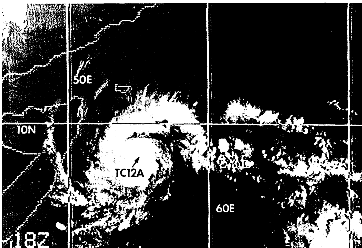
Figure 3-12A-1. At peak intensity, TC12A approaches the coast of Somalia (230500Z December DMSPI infrared imagery).
