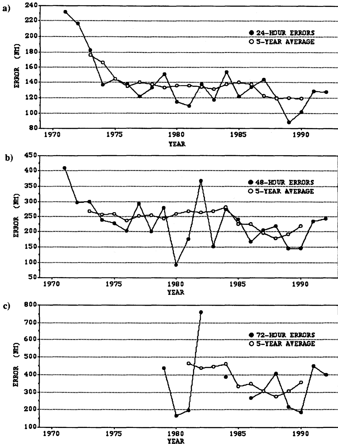
Figure 5-6. Mean track errors (nm) and 5-year running mean for a) 24 hours, b) 48 hours and c) 72 hours in the North Indian Ocean. Note: no 72-hour forecasts verified prior to 1979, in 1983 and 1985.
