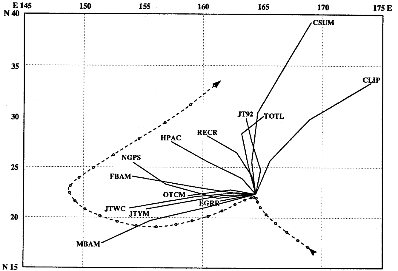
Figure 3-27-5. Forecast aids at 291200Z October for the major track change. Shown are the climatological/statistical forecast aids HPAC, CLIP, TOTL, RECR, JT92 and CSUM along with the dynamic aids OTCM, FBAM, MBAM, JTYM and the numerical models, NGPS and EGRR.
