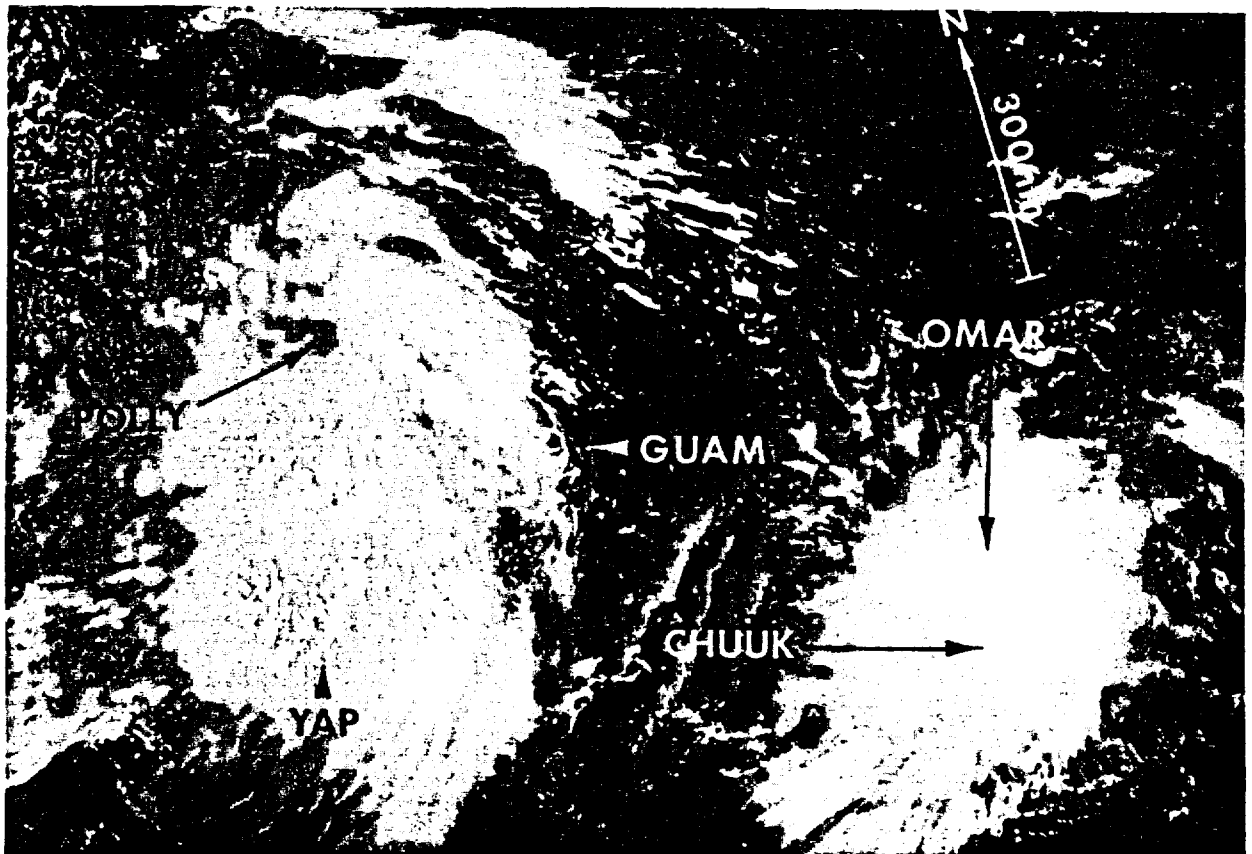
Figure 3-15-1. Omar Passes north of Chuuk as Polly (14W) consolidates to the west of Guam (242320Z August DMSP visual imagery).
