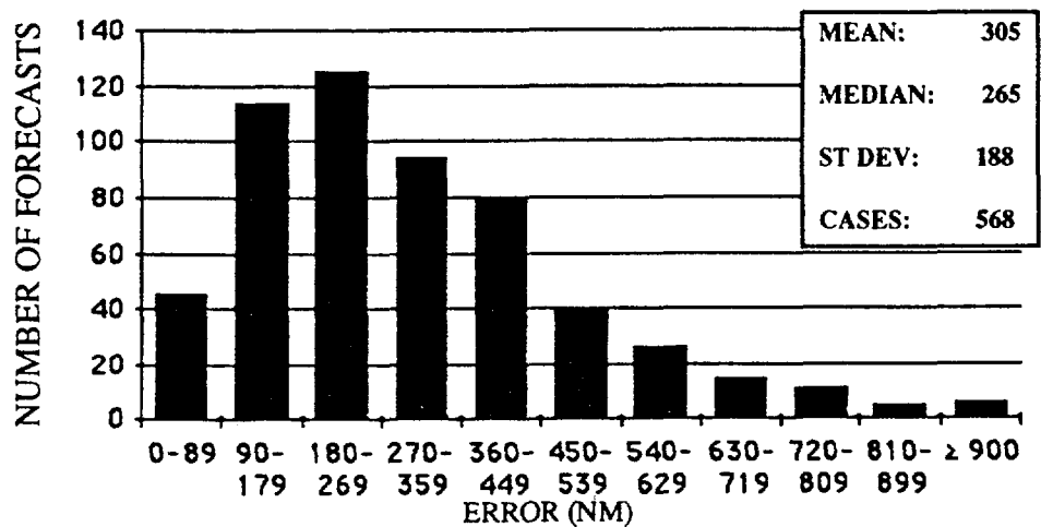
Figure 5-2f. Frequency distribution of 72-hour forecast errors (90 nm increments) for the western North Pacific Ocean in 1992. The largest error, 1014 nm, occurred on Typhoon Colleen (26W).
