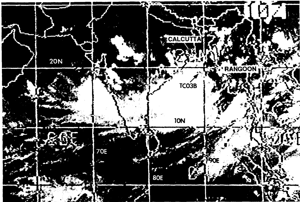
Figure 3-03B-1. TC03B a day before making landfall in India (161000Z - 161200Z June DMSPI infrared digitized mosaic).
