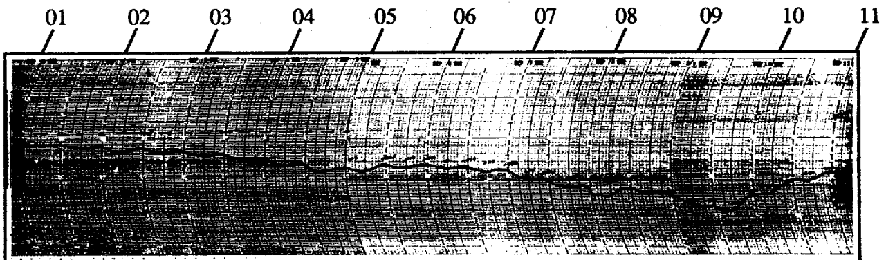
Figure 3-18-1. Barograph trace for the period 01-11 September for Wake Island (WMO 91245) showing the steadily falling pressures from 010000Z to 091445Z associated with the extension of the monsoon trough into the area, and the formation and intensification of Sibyl near the island. (Microbarograph trace courtesy of the National Weather Service Office, Wake Island).
