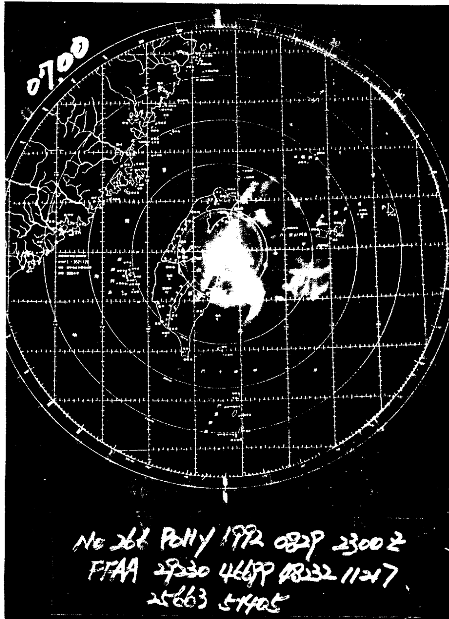
Figure 3-16-1. Although Polly is weakening, its eye remain's visible on the radar at Hualein (WMO 46699) (292300Z August radar photo courtesy of the Central weather Bureau, Taipei, Taiwan).
