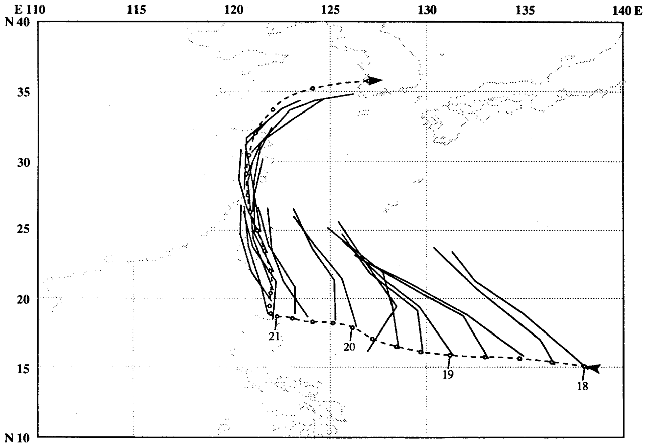
Figure 3-19-3. NOGAPS guidance for Ted is consistently north of track until the tropical storm enters the Luzon Strait, then the model locks on.
