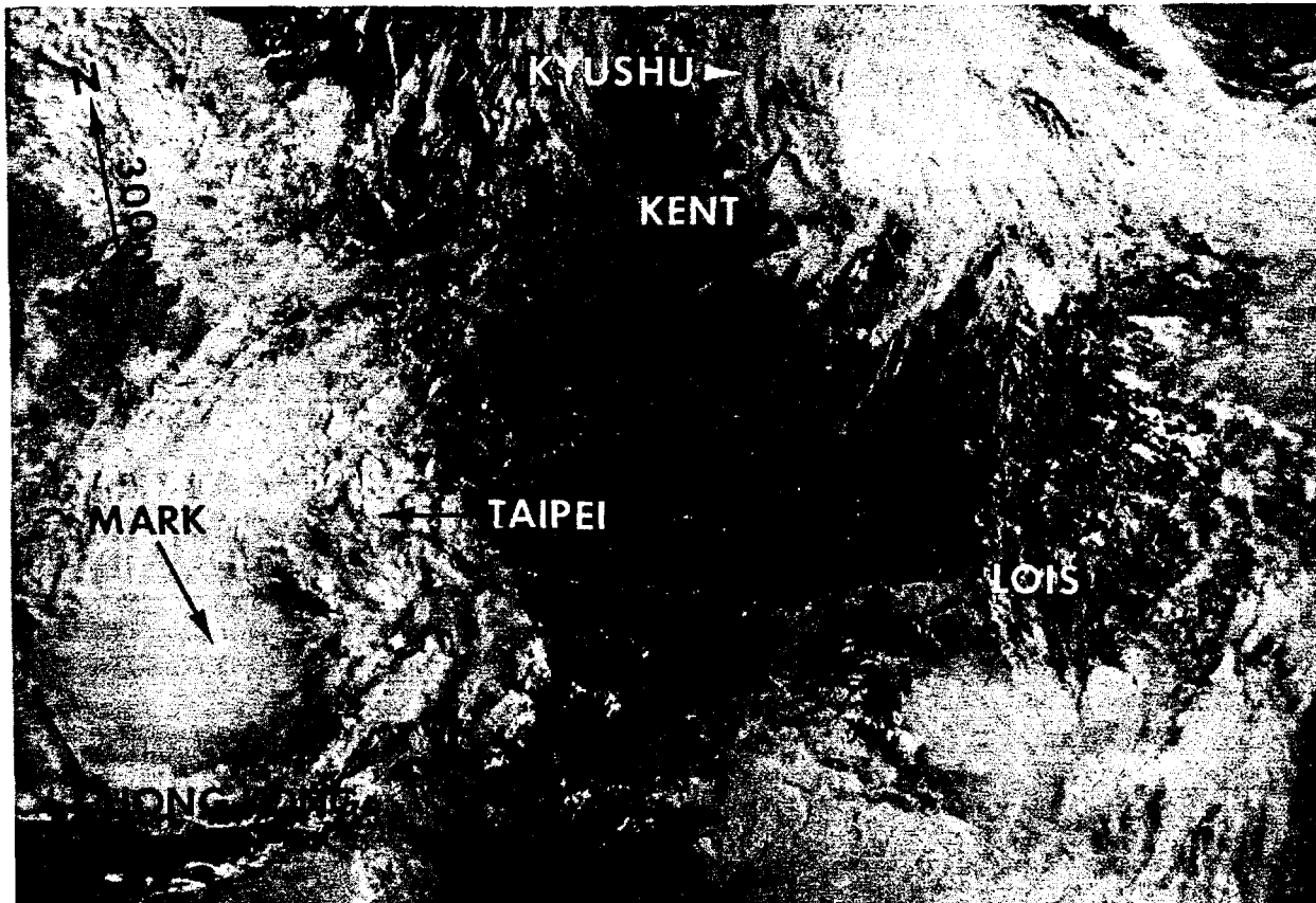
Figure 3-12-1. The partially exposed low-level circulation of Lois is visible to the south of Kent (11W) which is heading for Kyushu. To the west, Mark (13W) is churning up the South China Sea (172325Z August NOAA visual imagery).
