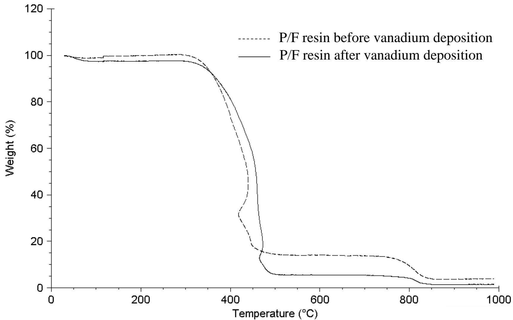
Figure 3 - TGA measurement under air (10°C/min) of the P/F resin
