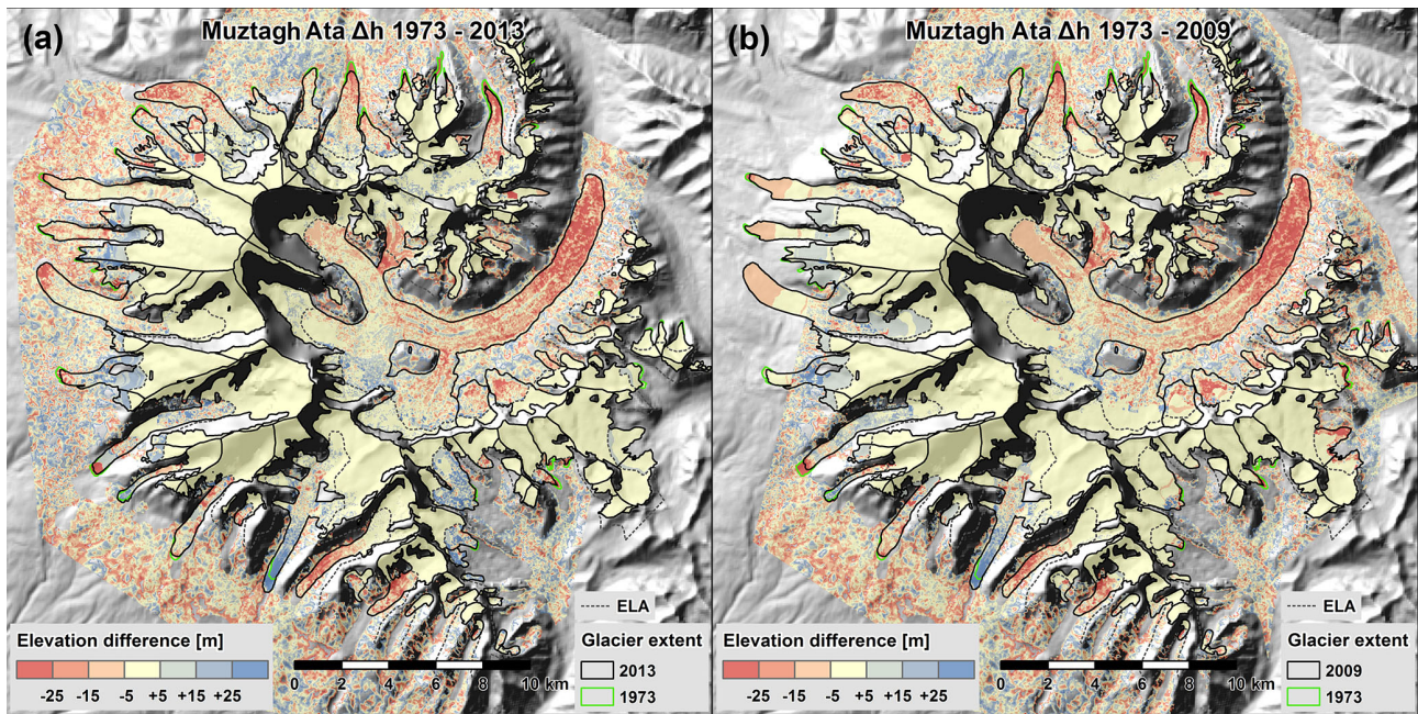
Figure 6. Co-registered map of elevation differences during 1973–2013 (a) and 1973–2009 (b) after outlier and gap-filling processing for glacier mass-balance and vertical uncertainty calculation.
