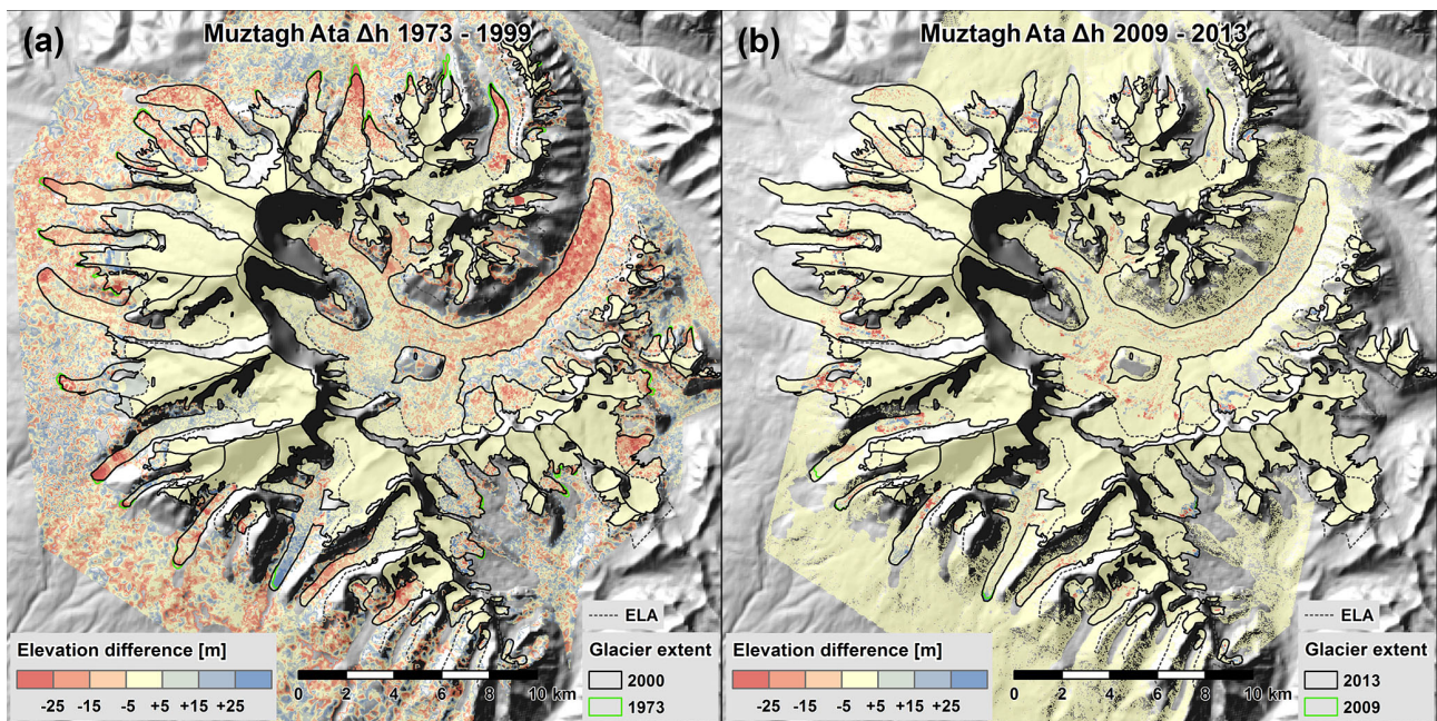
Figure 7. Co-registered map of elevation differences during 1973–1999 (a) and 2009–2013 (b) after outlier and gap-filling processing for glacier mass-balance and vertical uncertainty calculation.
