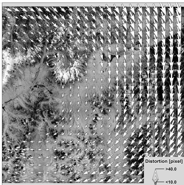
Figure 2. Distortion vectors of réseau crosses from their measured to their initial reference positions in a KH-9 photograph segment covering Muztagh Ata (frame 17a of mission 1206-5).
