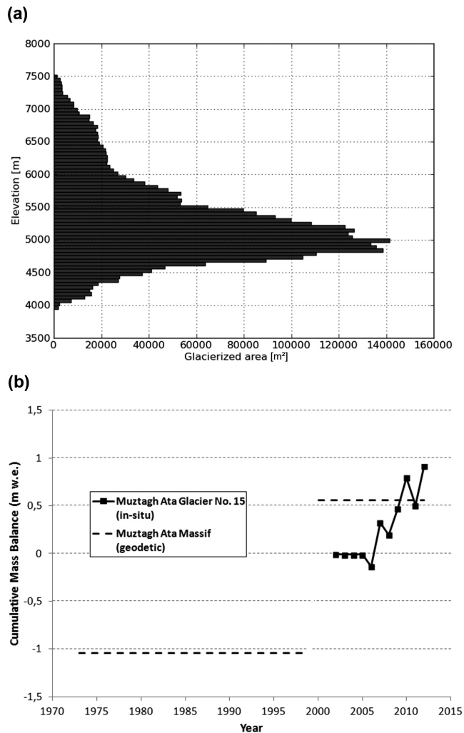
Figure 3. (a) Hypsometry of the glacierized area at Muztagh Ata, (b) cumulative glaciological mass balance of Muztagh Ata Glacier No. 15 (G075058E38248N) vs. cumulative geodetic mass balance of the entire Muztagh Ata Massif.
