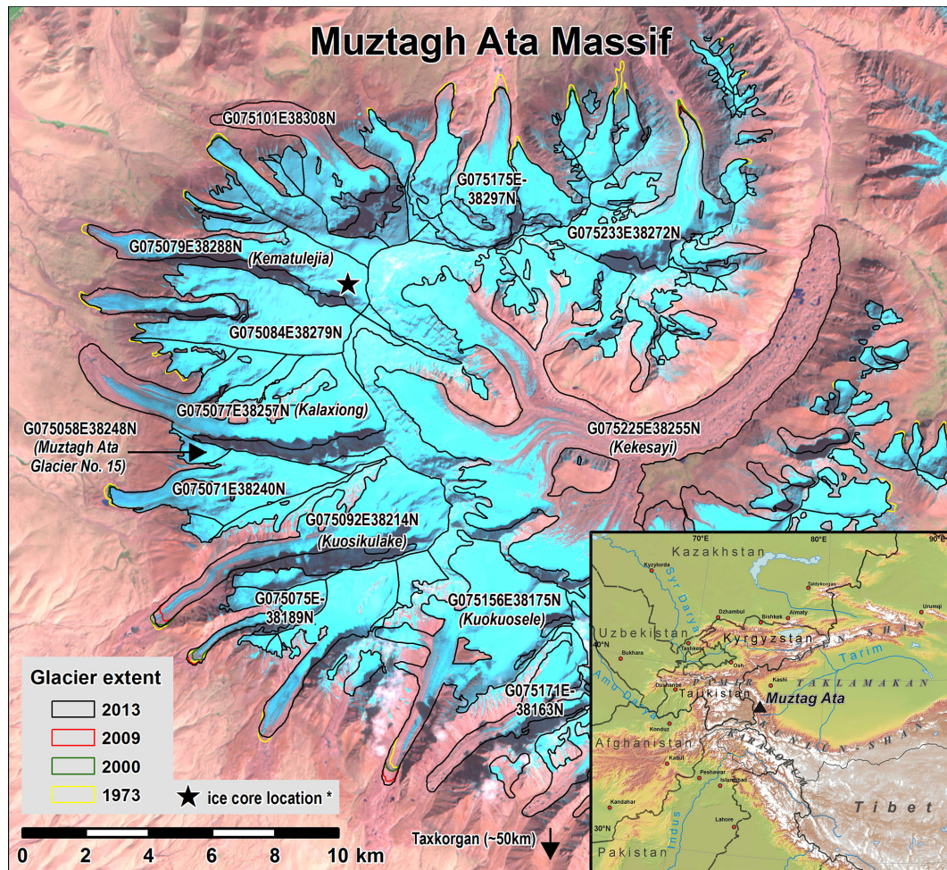
Figure 1. Overview of the Muztagh Ata study site with investigated glaciers according to their ID in GLIMS (background image: Landsat 7 ETM+ of 11 September 2000; *: ice core location Tian et al., 2006; Duan et al., 2007).
