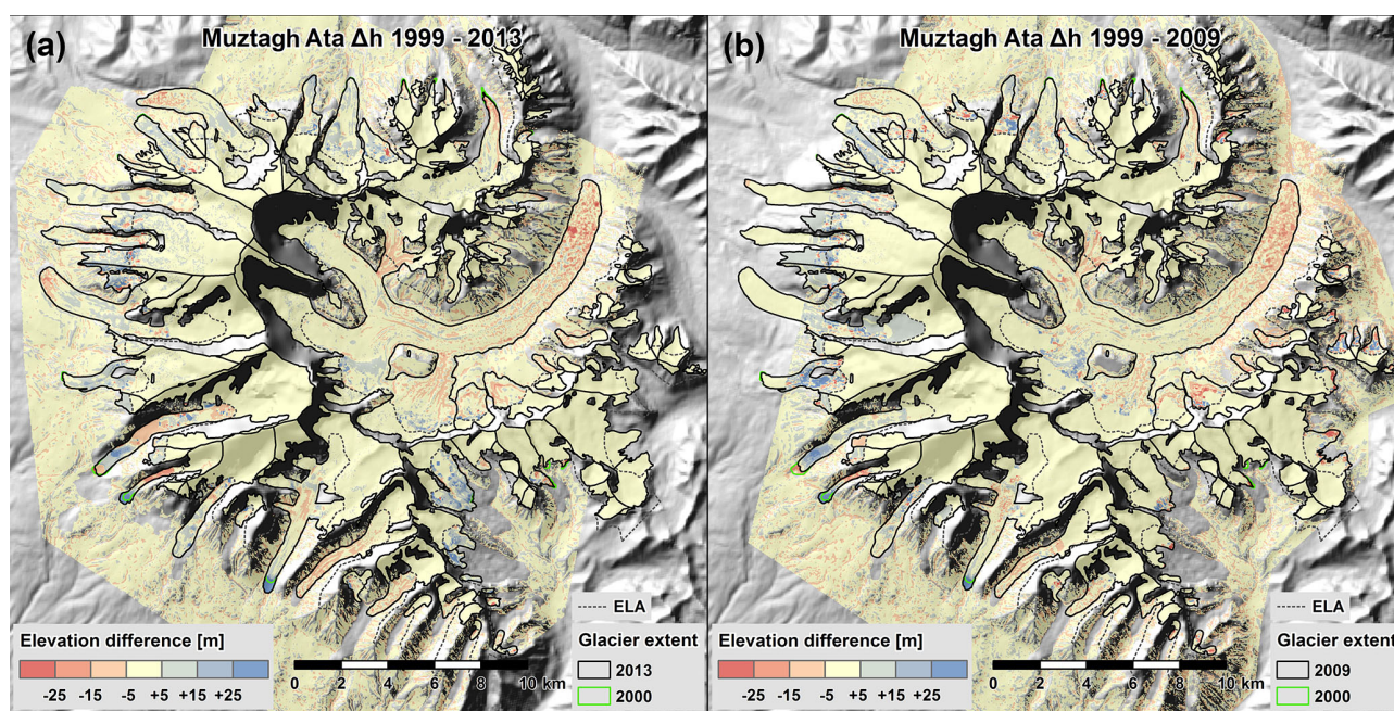
Figure 8. Co-registered map of elevation differences during 1999–2013 (a) and 1999–2009 (b) after outlier and gap-filling processing for glacier mass-balance and vertical uncertainty calculation.
