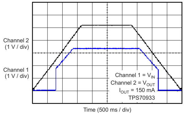
6-34. Power-Up and Power-Down Response
