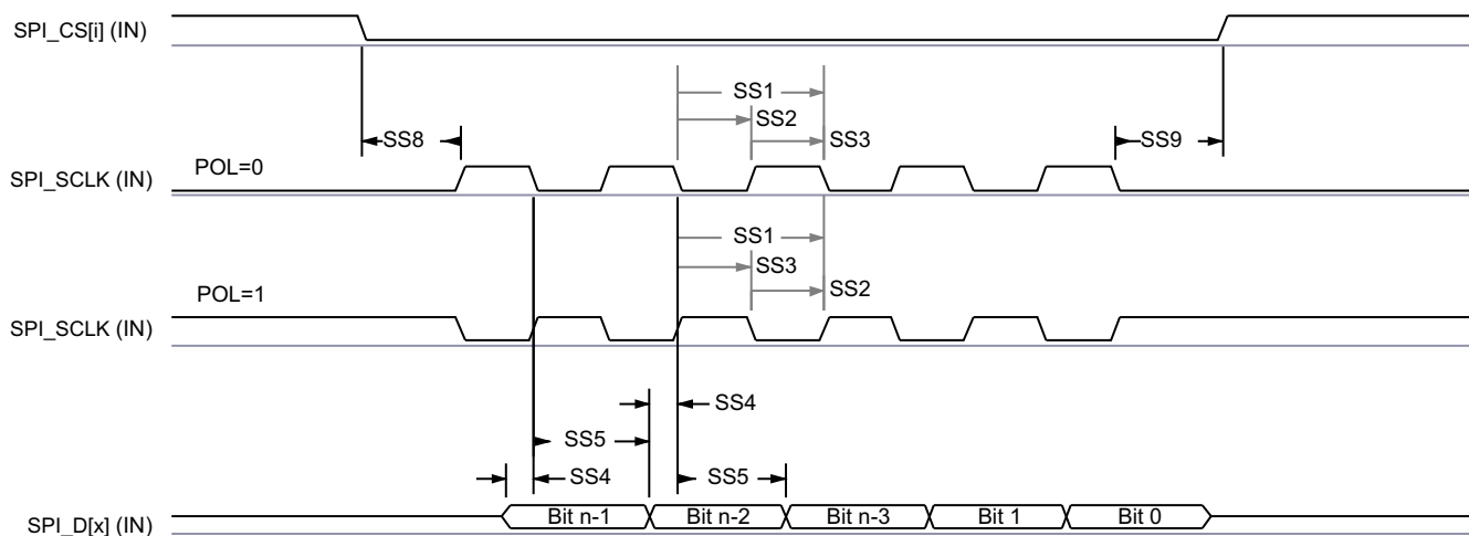
Figure 6-75. SPI Peripheral Mode Receive Timing
