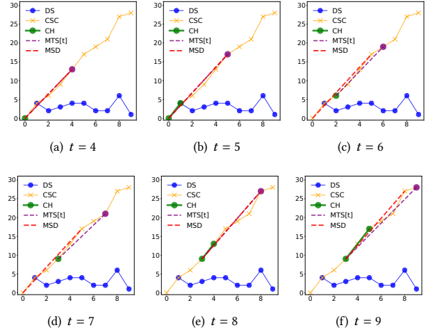
Figure 2: Running example of computing maximum l -segment density for a degree sequence of [4, 2, 3, 4, 4, 2, 2, 6, 1] with l = 4 . The data on x-axis and y-axis represent the time t and the cumulative sum.
