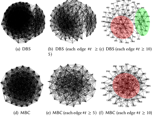
Figure 9: Communities results on Enron
