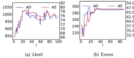
Figure 8: Effectiveness results of POMBCs
