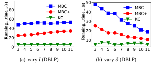
Figure 11: Running time (s) with varying l, \delta on DBLP
