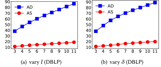
Figure 10: Effectiveness of MBC with varying l, \delta on DBLP
