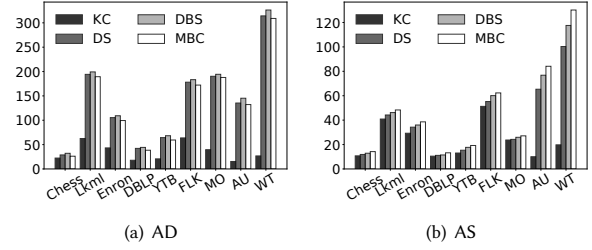
Figure 4: Effectiveness results of KC, DS and MBC
