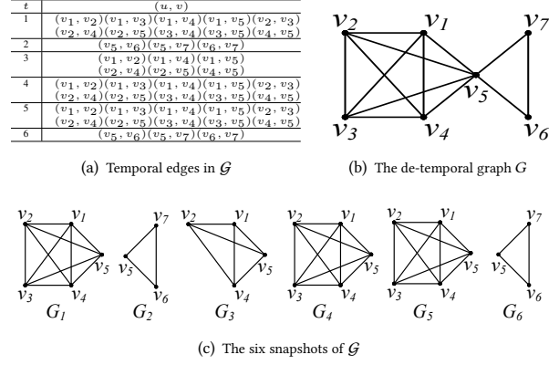
Figure 1: Basic concepts of the temporal graph
