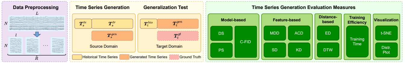
Figure 3: Overall architecture of TSGBench.
