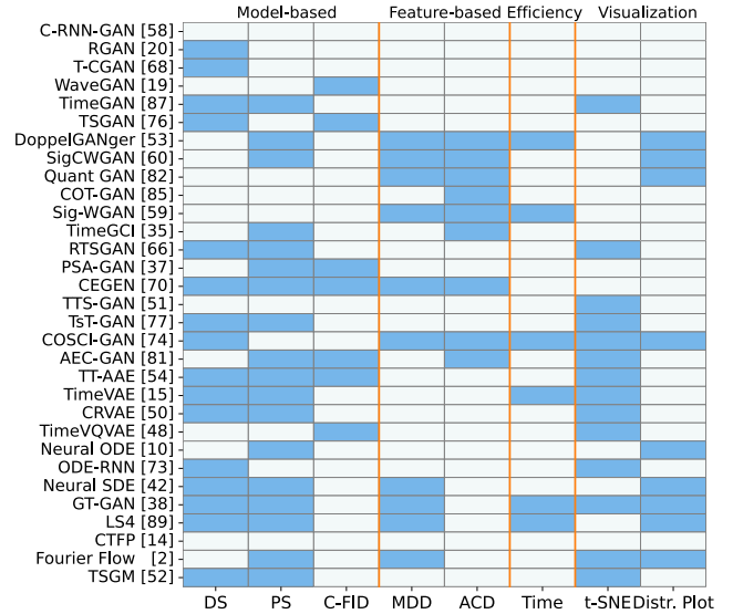
Figure 4: Summary of evaluations in popular TSG methods.
