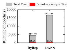
Figure 9: Ratio of dependency analysis time.
