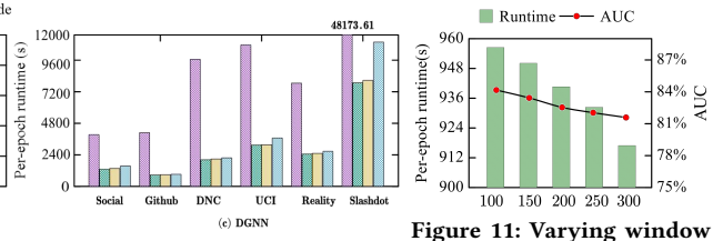
Figure 11: Varying window size in NS-Slide.
