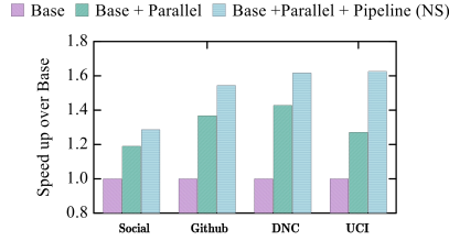
Figure 12: Performance breakdown analysis.
