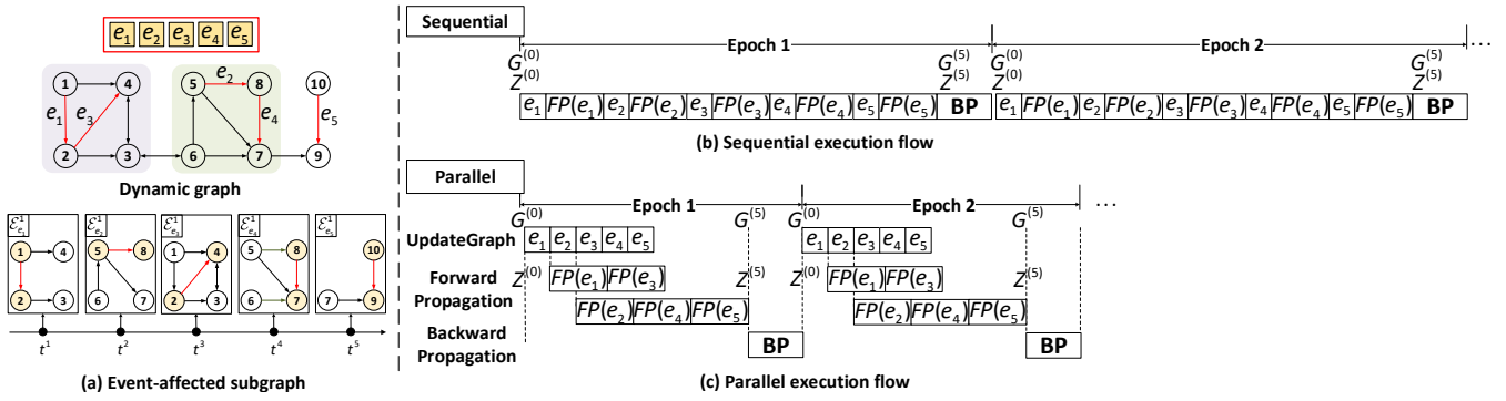
Figure 3: Execution flow comparison of sequential execution events and parallel execution events. The red arrows represent the newly added edge. FP represents forward propagation, while BP represents backward propagation. Figure (a) is the 1-hop event-affected subgraph \mathcal{E}_e^1 of event e_1, e_2, e_3, e_4, e_5 . The purple area is the affected subgraph of events e_1 and e_3 , and the green area is the affected subgraph of events e_2 and e_4 .
