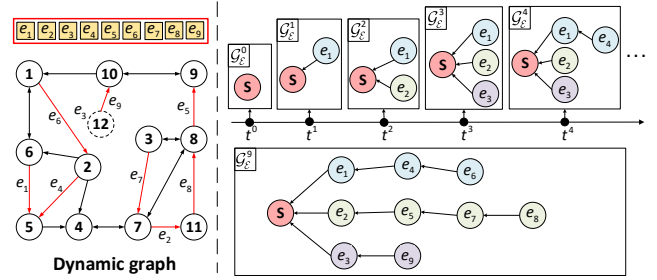
Figure 4: Event dependency graph. The red arrows represent the newly added edge, and the dotted line represents the newly added node. The upper right corner is the evolved Event Dependency Graph. The lower right corner is the complete event dependency graph, where nodes of the same color represent a dependency chain.
