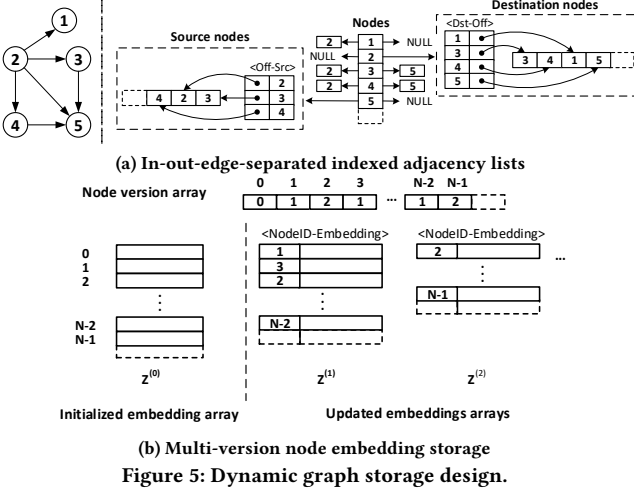
Figure 5: Dynamic graph storage design.
